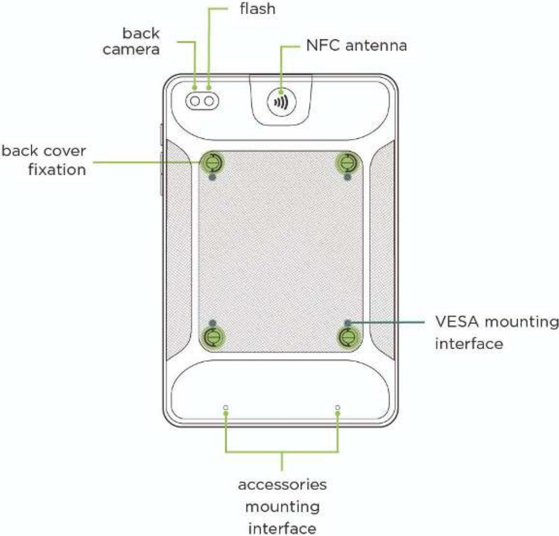
back view
